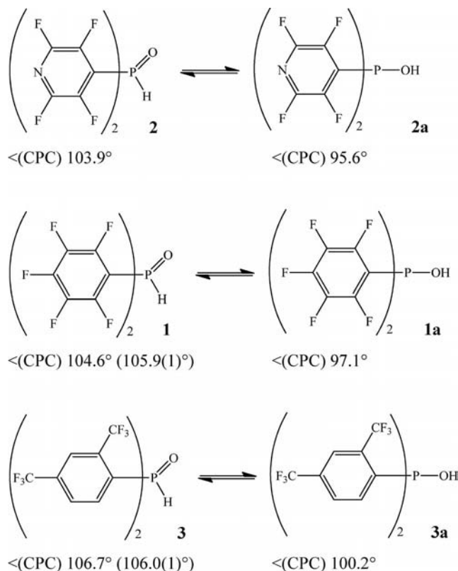
Scheme 3. Experimental (in brackets) and calculated [B3LYP/6-311G(2d,p)] C–P–C angles of the diarylphosphane oxides 1–3 and the corresponding phosphinous acids 1a–3a .
