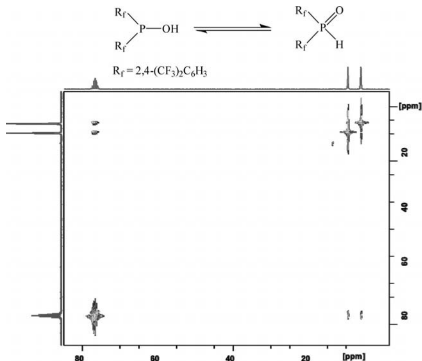
Figure 3. 2D ^{31}\text{P} EXSY NMR spectrum of bis[2,4-bis(trifluoromethyl)phenyl]phosphane oxide ( 3 ) in [\text{D}_6]\text{DMSO} at room temp.
