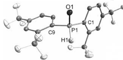
Figure 1. Molecular structure of bis[2,4-bis(trifluoromethyl)phenyl]phosphane oxide ( 3 ) (ellipsoids are drawn at 50% probability level; all C-bonded hydrogen atoms have been omitted for clarity). Selected bond lengths [pm] and angles [°]: P1–O1 148.5(1), P1–C1 181.7(2), P1–H1 1.29(2), P1–C9 182.3(2), C1–P–C9 106.0(1).
