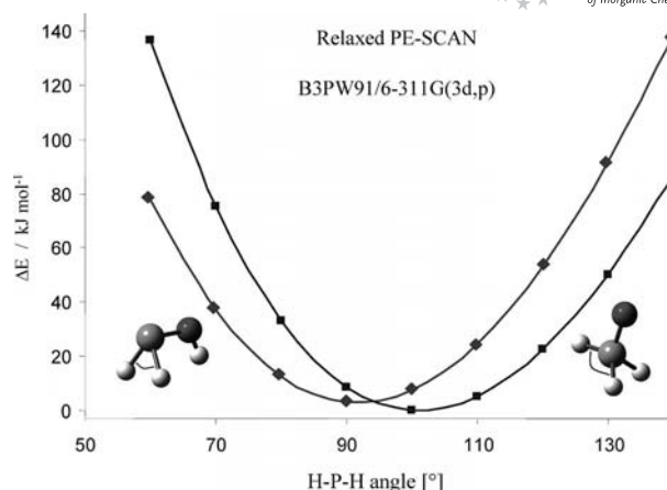
Figure 4. Dependence of the potential energies of \text{H}_2\text{P–OH} and \text{H}_3\text{PO} on the H–P–H angle [relaxed potential energy scan at the B3PW91/6-311G(3d,p) level of theory].
