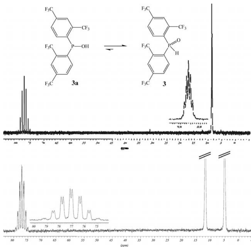
Figure 2. ^{31}\text{P}\{^1\text{H}\} NMR (top) and ^{31}\text{P} NMR (bottom) spectra of the tautomeric phosphane oxide 3 and the corresponding phosphinous acid 3a in [\text{D}_6]\text{DMSO} at room temp.
