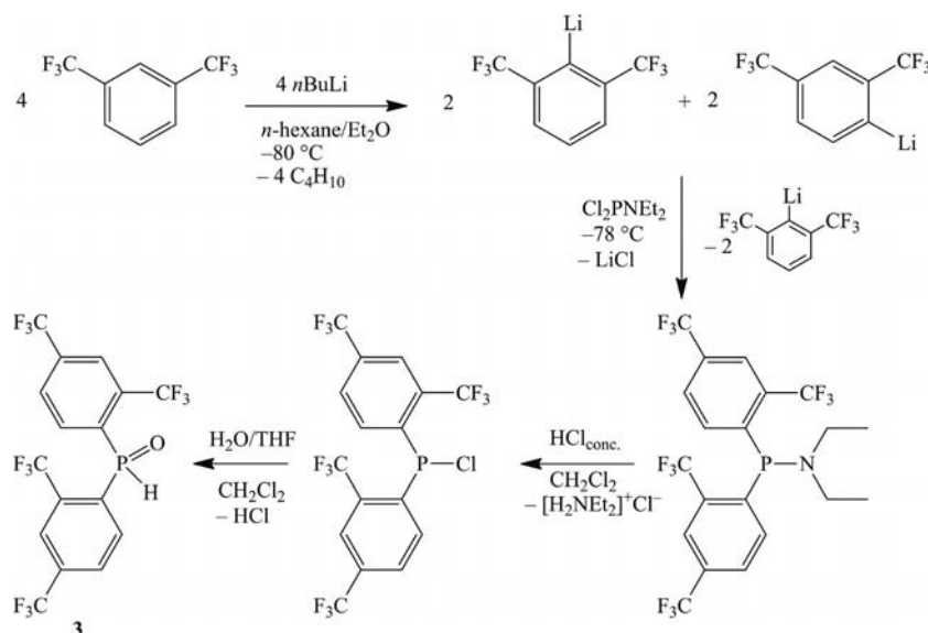
Scheme 2. Reaction of dichloro(diethylamino)phosphane with lithiated 1,3-bis(trifluoromethyl)benzene, P–N bond cleavage to the intermediate chlorophosphane, and its eventual hydrolysis to bis[2,4-bis(trifluoromethyl)phenyl]phosphane oxide ( 3 ).
