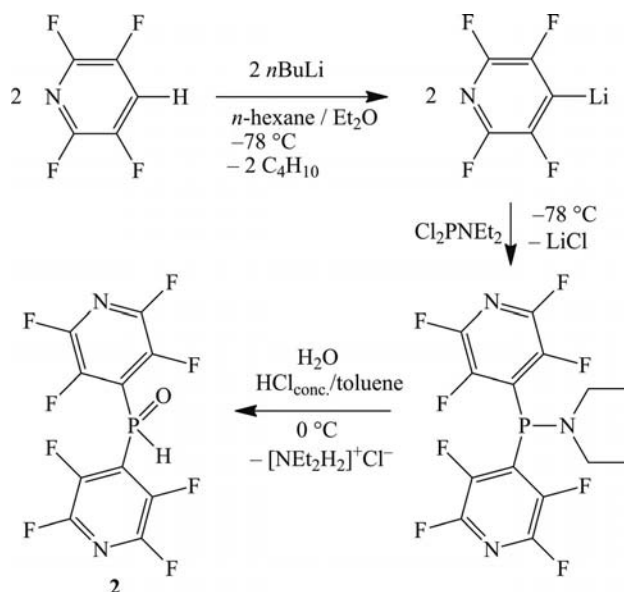
Scheme 1. Reaction of dichloro(diethylamino)phosphane with lithiated tetrafluoropyridine and subsequent hydrolysis of the intermediate to give bis(tetrafluoropyridyl)phosphane oxide ( 2 ).
